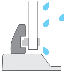
bottom framed shower enclosures 10°, Pivot, Blix Slim, Blix, Supernova
