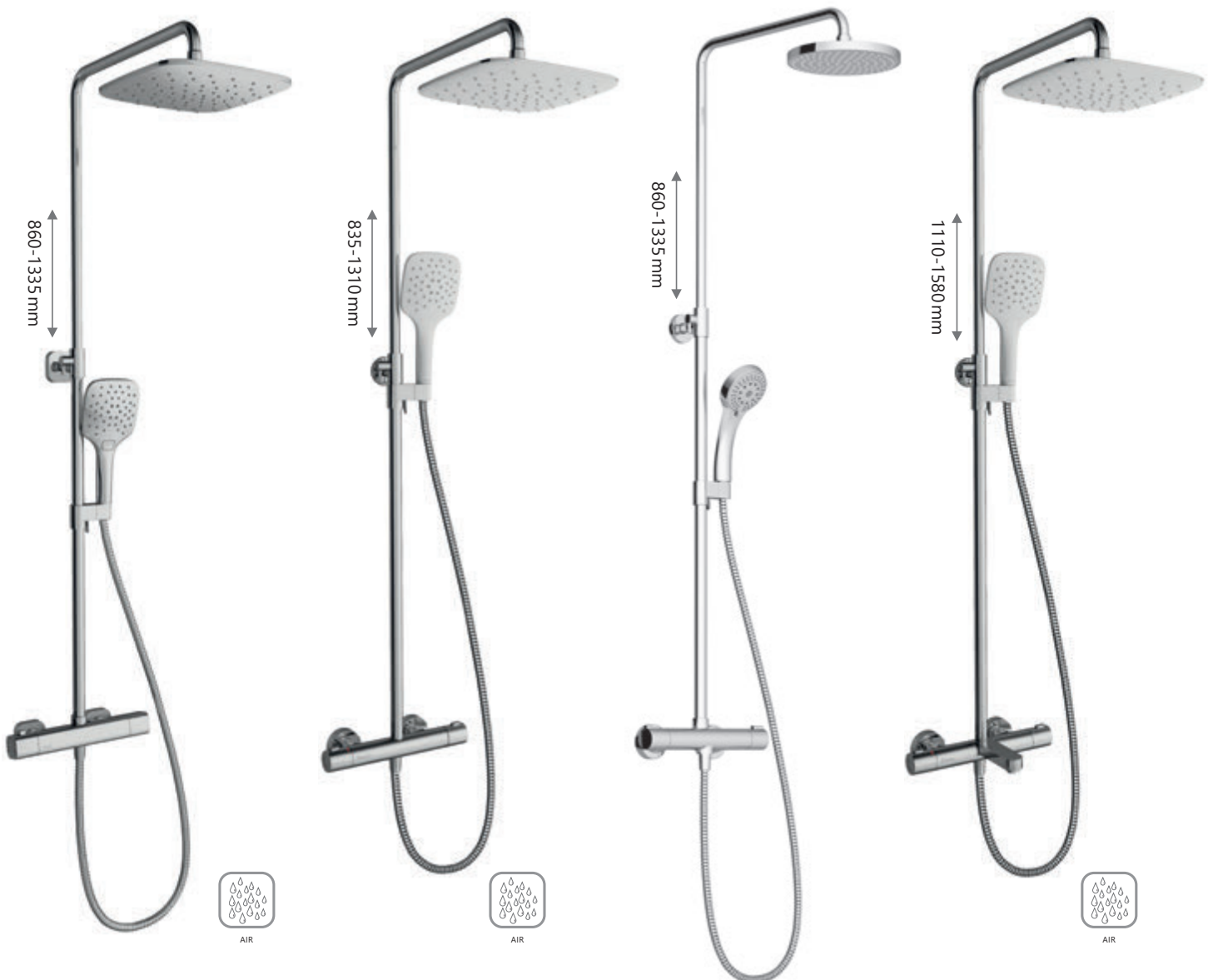
Shower column 10°, with thermostatic faucet and shower set, chrome TD 091.00/150 Order No. X070103
