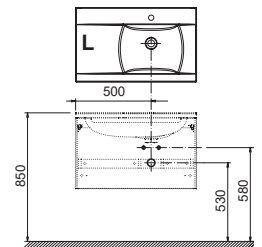
SD Classic II 800 L
